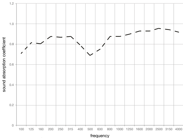
NRC for ScreenTrak® Bass is using results for 0.47" ecoustic® Screen with a 11.8" airgap ScreenTrak® Bass (NRC .85)
